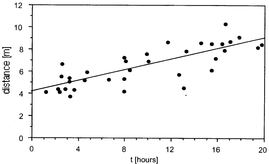
Fig. 1. Regression between the time since the spider had built a previous web ( \Delta t ) and investment into the web expressed as the distance the spider had walked to build the capture spiral ( y = 4.16 + 0.24x , r^2 = 0.637 , p < 0.0001 , n = 35 ). Only webs where the time since the previous web ( \Delta t ) was less than 20 hours were used in this analysis.
