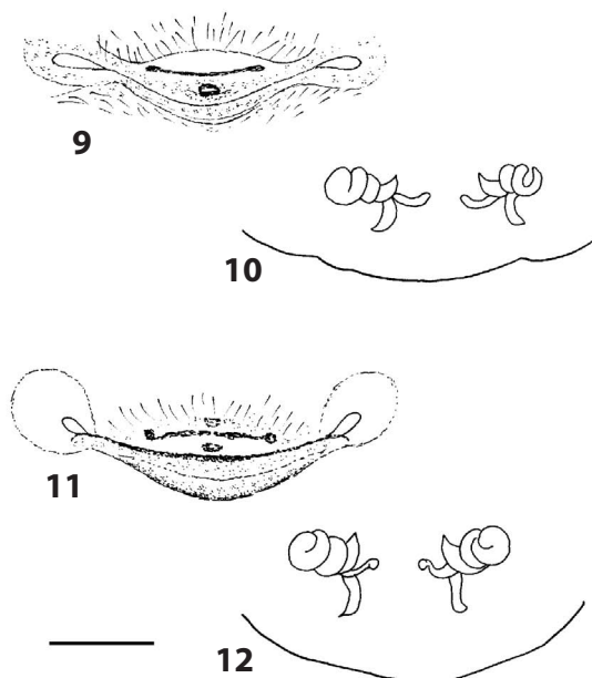
Figures 9-12: Zangherella relicta : 9 – epigyne; 10 – vulva, dorsal (Herceg Novi); 11 – epigyne; 12 – vulva, dorsal (Pirin Mts.). Scale bar: 0.15 mm.
