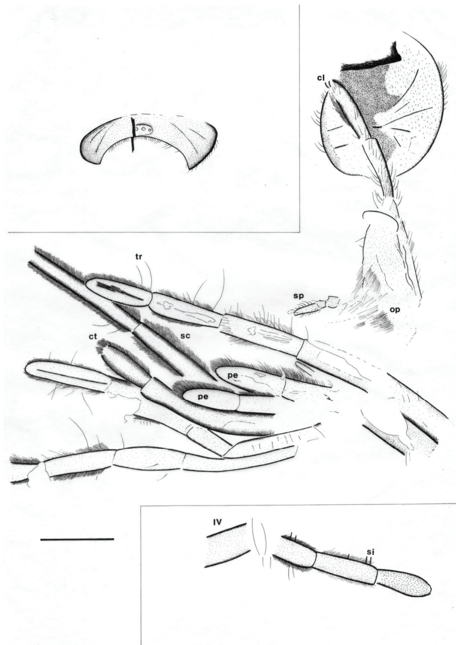
Fig. 9. Camera lucida drawing of the specimen shown in Figs 2–8. Insets show carapace and probable fourth leg. Abbreviations: IV = probable fourth leg; cl = tarsal claws; ct = claw tuft; op = opisthosomal cuticle; pe = pedipalp; sc = scopulae; si = possible spines on leg; sp = spinneret; tr = trichobothria. Scale bar equals 5 mm.
