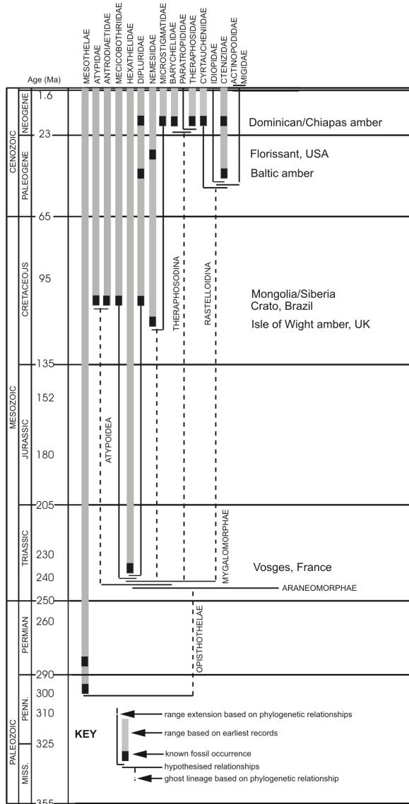
Fig. 1. Evolutionary tree of the mygalomorph families (Araneae: Mygalomorphae). Cladogram superimposed on the known fossil record. Emended and updated from Penney et al. (2003, fig. 1) who detail the sources and methods used in its construction. The approximate stratigraphical position and age of the localities mentioned in Table 1 is indicated, with the exception of Aix-en-Provence and the Palaeogene of the Isle of Wight, whose fossils cannot be placed with confidence in any family.
